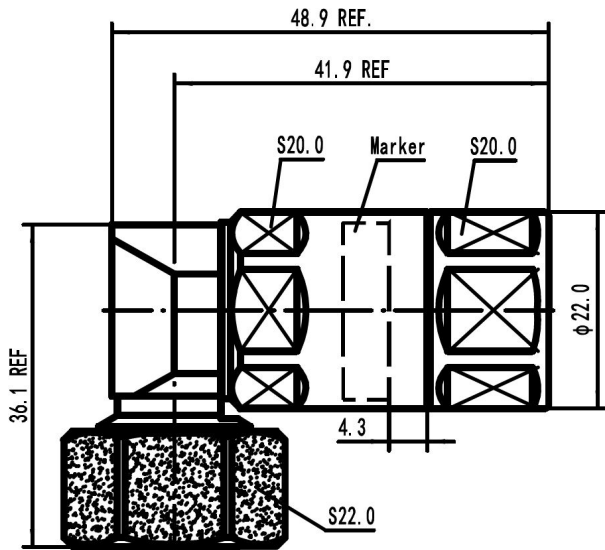
43MR-LCF12-C03 Outline drawing
